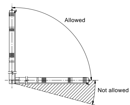
Fig. 4 Installation of SQF pumps
